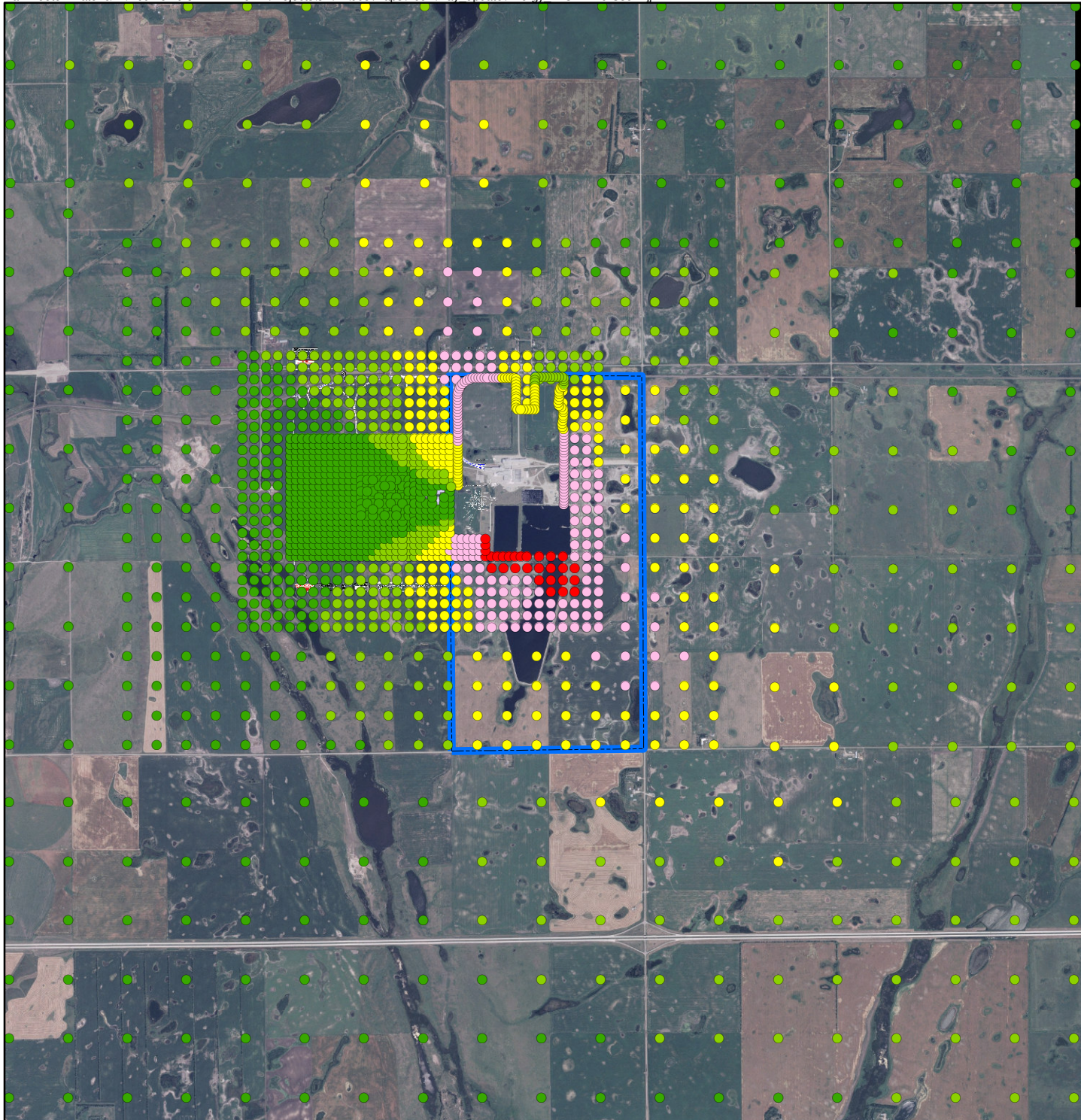
Figure D-2 Combined Risk for Group 1&2 HAPs with 30/70 Factor Applied
