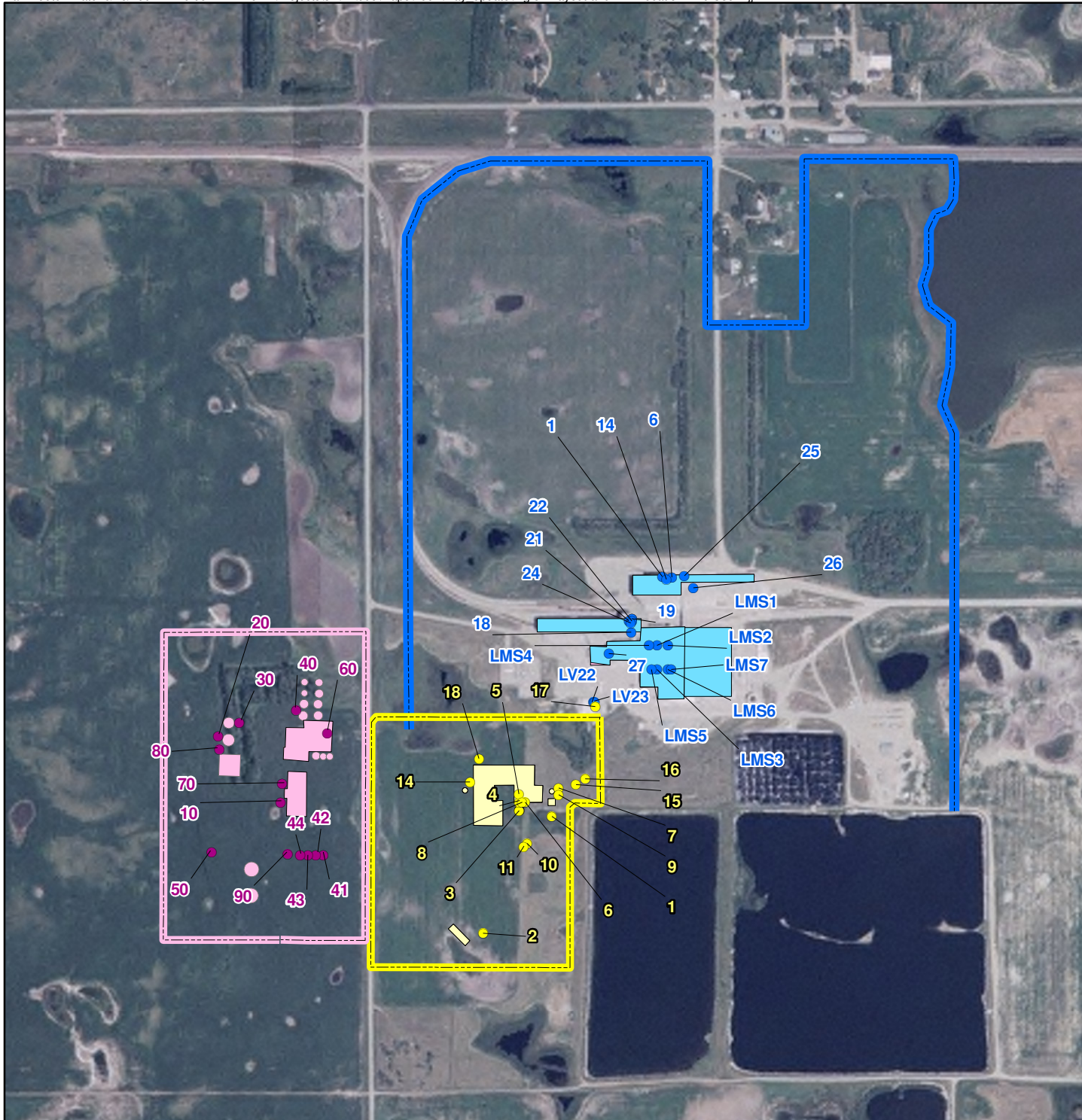
Figure 3 Facility Layout and Stack Locations
